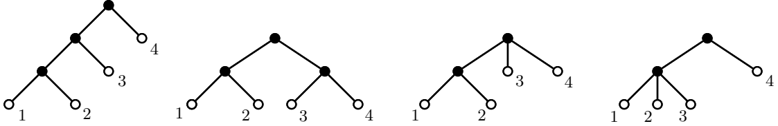
FIGURE 1. Simplices in T_4
